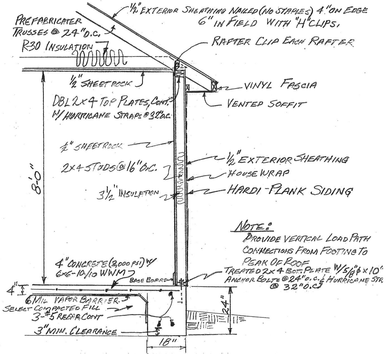
TYPICAL EXTERIOR WALL SECTION & FOOTING
